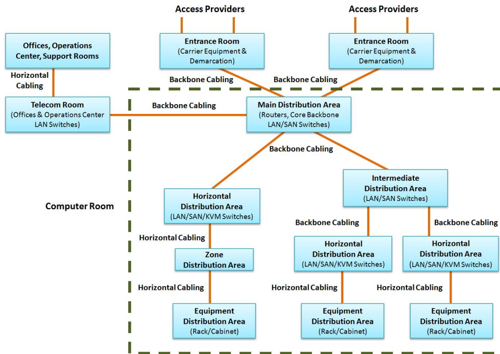
Figure 1: TIA-942-A Data Center Topology (similar to ISO 24764)
